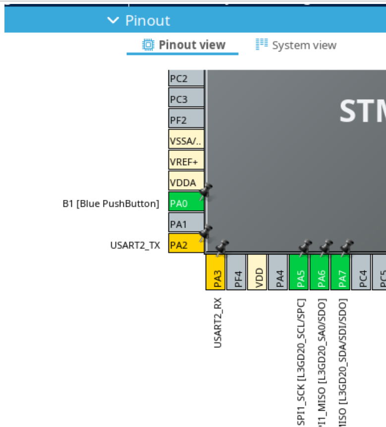
Figure 7.4: TX/RX Pins
